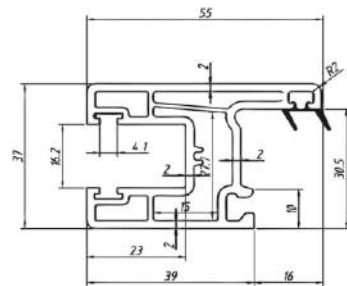
SECTION NAME- SLIDING WINDOW SASH CODE - 103 WEIGHT - 0.840 KG/MTR STANDARD PACKAGES- 8 Pcs. (STD-8)
