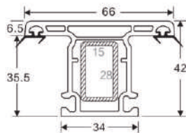
42 SASH SLIDING MULLION 2 Code: SB-42SM WEIGHT(KG/M): 0.84 LENGTH: 5.9 M (STD-8)
