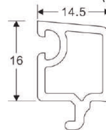
SLIDING 12 MM GLASS BEAD Code: SB-2001 WEIGHT(KG/M): 0.18 LENGTH: 5.9 M (STD-30)
