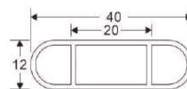
BLIND LOUVER Code: SB-CLP WEIGHT(KG/M): 0.217 LENGTH: 5.9 M (STD-20)
