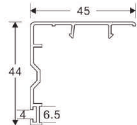
92 SLIDING DOOR SASH COVER Code: SB-2005 WEIGHT(KG/M): 0.227 LENGTH: 5.9 M (STD-20)
