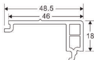
SHUTTER GLAZING BEAD Code: SB-SGB WEIGHT(KG/M): 0.26 LENGTH: 5.9 M (STD-20)
