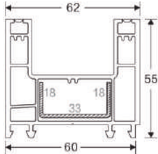
2- TRACK OUTER FRAME Code: SB-1001 WEIGHT(KG/M): 1.10 LENGTH: 5.9 M (STD-6)
