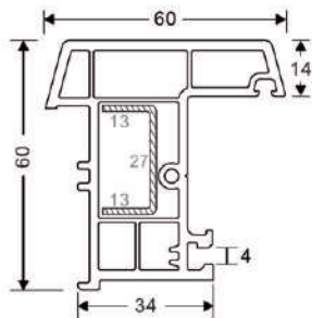
FRENCH MULLION / LAP JOINT Code: SB-3005 WEIGHT(KG/M): 1.067 LENGTH: 5.9 M (STD-6)
