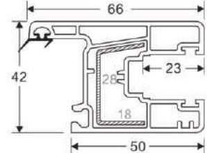
66 SLIDING WINDOW SASH Code: SB-1004 WEIGHT(KG/M): 1.062 LENGTH: 5.9 M (STD-8)
