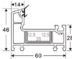
60 OUT WARD DOOR SASH Code: SB-3003 WEIGHT(KG/M): 1.69 LENGTH: 5.9 M (STD-4)
