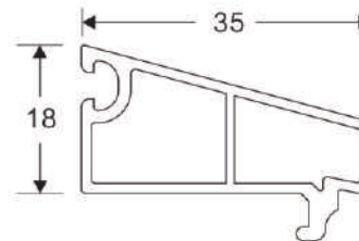
60 OUT WARD DOOR SASH Code: SB-3003 WEIGHT(KG/M): 1.69 LENGTH: 5.9 M (STD-4)
