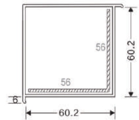
60 RIGHT ANGLE BAY CORNER ADAPTOR Code: SB-C90 WEIGHT(KG/M): 0.71 LENGTH: 5.9 M (STD-4)
