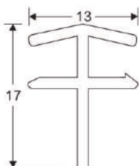
FRAME CONNECTOR Code: SB-F1 WEIGHT(KG/M): 0.092 LENGTH: 5.9 M (STD-50)
