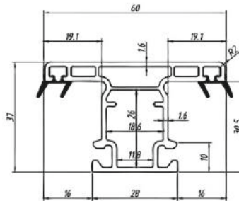
SECTION NAME- SLIDING MULLION CODE - 105 WEIGHT - 0.59 KG/MTR STANDARD PACKAGES- 8 Pcs. (STD-8)
