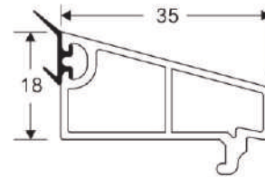
60 MULLION CASMENT Code: SB-3004 WEIGHT(KG/M): 1.10 LENGTH: 5.9 M (STD-6)
