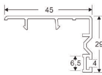
66 SLIDING WINDOW SASH COVER Code: SB-2004 WEIGHT(KG/M): 0.217 LENGTH: 5.9 M (STD-20)
