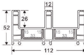
112 SLIDING FRAME-3T Code: SB-1003 WEIGHT(KG/M): 1.750 LENGTH: 5.9 M (STD-4)
