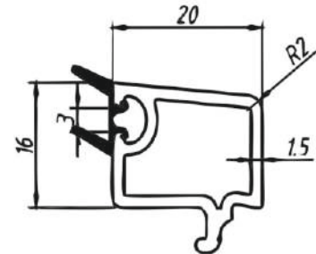
SECTION NAME- SINGLE GLAZING BEAD CODE - 106 WEIGHT - 0.22 KG/MTR STANDARD PACKAGES- 20 Pcs. (STD-20)
