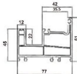
MONORAIL/SLIDING FRAME Code: SB-M1 WEIGHT(KG/M): 1.24 LENGTH: 5.9 M (STD-6)
