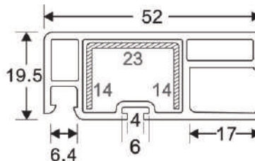
52 SCREEN DOOR SASH Code: SB-1007 WEIGHT(KG/M): 0.506 LENGTH: 5.8-6 Om (STD-9)
