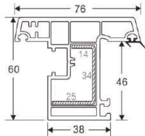
60 OUT WARD WINDOW SASH Code: SB-3002 WEIGHT(KG/M): 1.230 LENGTH: 5.9 M (STD-6)
