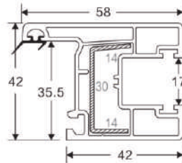
58 SLIDING SASH D Code: SB-1006 WEIGHT(KG/M): 0.84 LENGTH: 5.9 M (STD-8)
