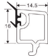
SLIDING 12 MM GLASS BEAD Code: SB-2001 WEIGHT(KG/M): 0.18 LENGTH: 5.9 M (STD-30)
