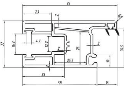
SECTION NAME- SLIDING DOOR SASH CODE - 104 WEIGHT - 1.02 KG/MTR STANDARD PACKAGES- 6 Pcs. (STD-6)
