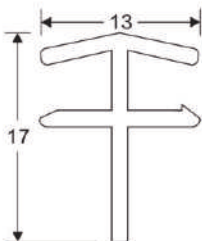
FRAME CONNECTOR Code: SB-F1 WEIGHT(KG/M): 0.092 LENGTH: 5.9 M (STD-50)
