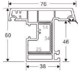
60 OUT WARD WINDOW SASH Code: SB-3002 WEIGHT(KG/M): 1.230 LENGTH: 5.9 M (STD-6)
