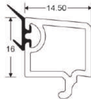
22MM GLAZING BEAD Code: SB-4003 WEIGHT(KG/M): 0.209 LENGTH: 5.9 M (STD-30)
