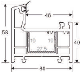
60 CASMENT OUTER FRAME Code: SB-3001 WEIGHT(KG/M): 1.01 LENGTH: 5.9 M (STD-6)
