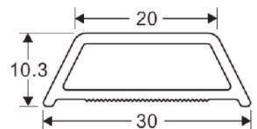
30 MM D. STRIP Code: SB-D1 WEIGHT(KG/M): 0.16 LENGTH: 5.9 M (STD-30)
