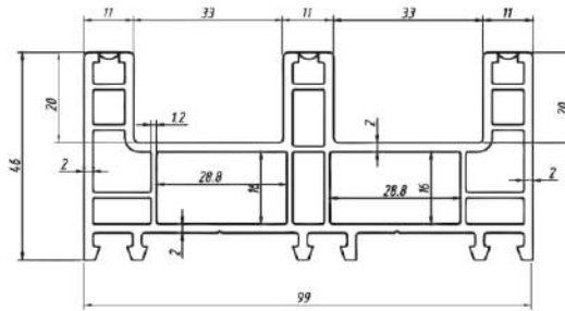
SECTION NAME- 3 TRACK CODE - ECO 102 WEIGHT- 1.42 KG/MTR STANDARD PACKAGES- 4 Pcs. (STD-4)
