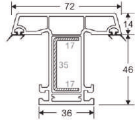
60 MULLION CASMENT Code: SB-3004 WEIGHT(KG/M): 1.10 LENGTH: 5.9 M (STD-6)
