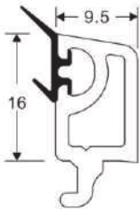
SLIDING 22 MM GLASS BEAD Code: SB-2002 WEIGHT(KG/M): 0.150 LENGTH: 5.9 M (STD-30)
