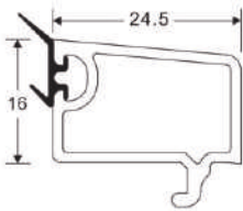
CASEMENT 12MM GLASS BEAD Code: SB-4002 WEIGHT(KG/M): 0.27 LENGTH: 5.9 M (STD-20)
