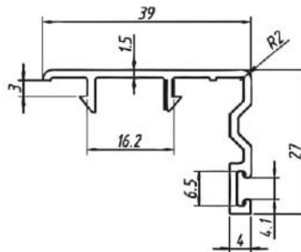
SECTION NAME- INTERLOCK CODE - 107 WEIGHT - 0.185 KG/MTR STANDARD PACKAGES- 20 Pcs. (STD-20)
