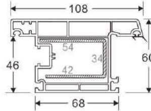
60 OUT WARD DOOR SASH Code: SB-3003 WEIGHT(KG/M): 1.69 LENGTH: 5.9 M (STD-4)
