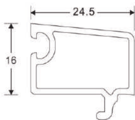
CASEMENT 12MM GLASS BEAD Code: SB-4002 WEIGHT(KG/M): 0.27 LENGTH: 5.9 M (STD-20)
