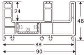
90 SLIDING FRAME 2.5 TRACK Code: SB-1002 WEIGHT(KG/M): 1.400 LENGTH: 5.9 M (STD-6)
