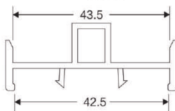
IN-LINE ADEPTOR Code: SB-2006 WEIGHT(KG/M): 0.307 LENGTH: 5.9 M (STD-10)
