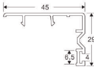
66 SLIDING WINDOW SASH COVER Code: SB-2004 WEIGHT(KG/M): 0.217 LENGTH: 5.9 M (STD-20)
