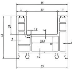
SECTION NAME- 2 TRACK CODE - 101 WEIGHT - 0.930 KG/MTR STANDARD PACKAGES- 6 Pcs. (STD-8)
