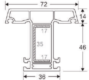
60 MULLION CASMENT Code: SB-3004 WEIGHT(KG/M): 1.10 LENGTH: 5.9 M (STD-6)
