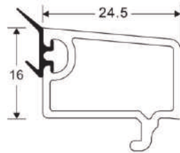
SLIDING SINGLE GALZED BEAD Code: SB-2003 WEIGHT(KG/M): 0.270 LENGTH: 5.9 M (STD-20)
