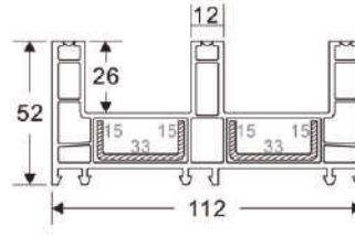
112 SLIDING FRAME-3T Code: SB-1003 WEIGHT(KG/M): 1.750 LENGTH: 5.9 M (STD-4)
