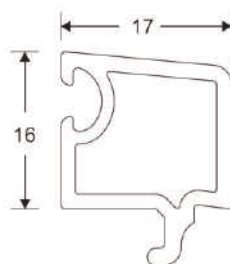
22MM GLAZING BEAD Code: SB-4003 WEIGHT(KG/M): 0.209 LENGTH: 5.9 M (STD-30)
