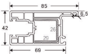
85 SLIDING DOOR SASH 2 Code: SB-1005 WEIGHT(KG/M): 1.22 LENGTH: 5.9 M (STD-4)
