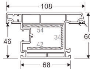
60 OUT WARD DOOR SASH Code: SB-3003 WEIGHT(KG/M): 1.69 LENGTH: 5.9 M (STD-4)
